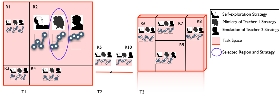
Figure 4: Selection of outcome and strategy is based on a partition of the outcome space with respect to different competence progress levels. We illustrate with the case of an outcome space of 3 different types of outcomes. T = T1 \cup T2 \cup T3 where T1 \subset R^2 , T2 \subset R and T3 \subset R^3 . T is partitioned in regions R_i for which are associated measures of competences \gamma for each strategy. The selection of outcome and strategy chooses the (region, strategy) pair that makes the most competence progress.
