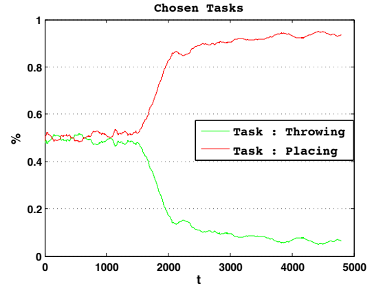
Figure 9: Outcome chosen by SGIM-ACTS through time, plotted as a mean percentage of several runs of the experiment.
